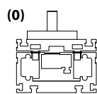
internal profile with cover bands
